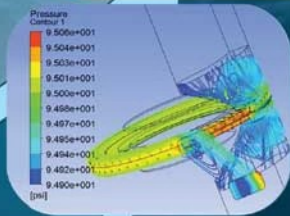
CFD analysis for repair validation
